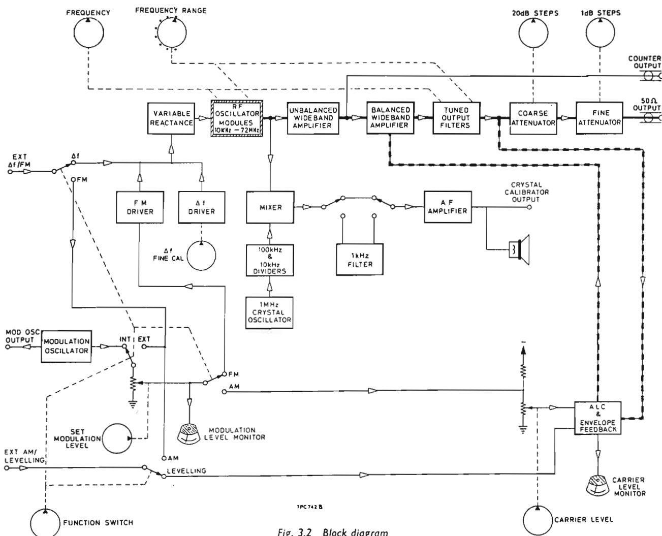
Fig. 3.2 Block diagram
