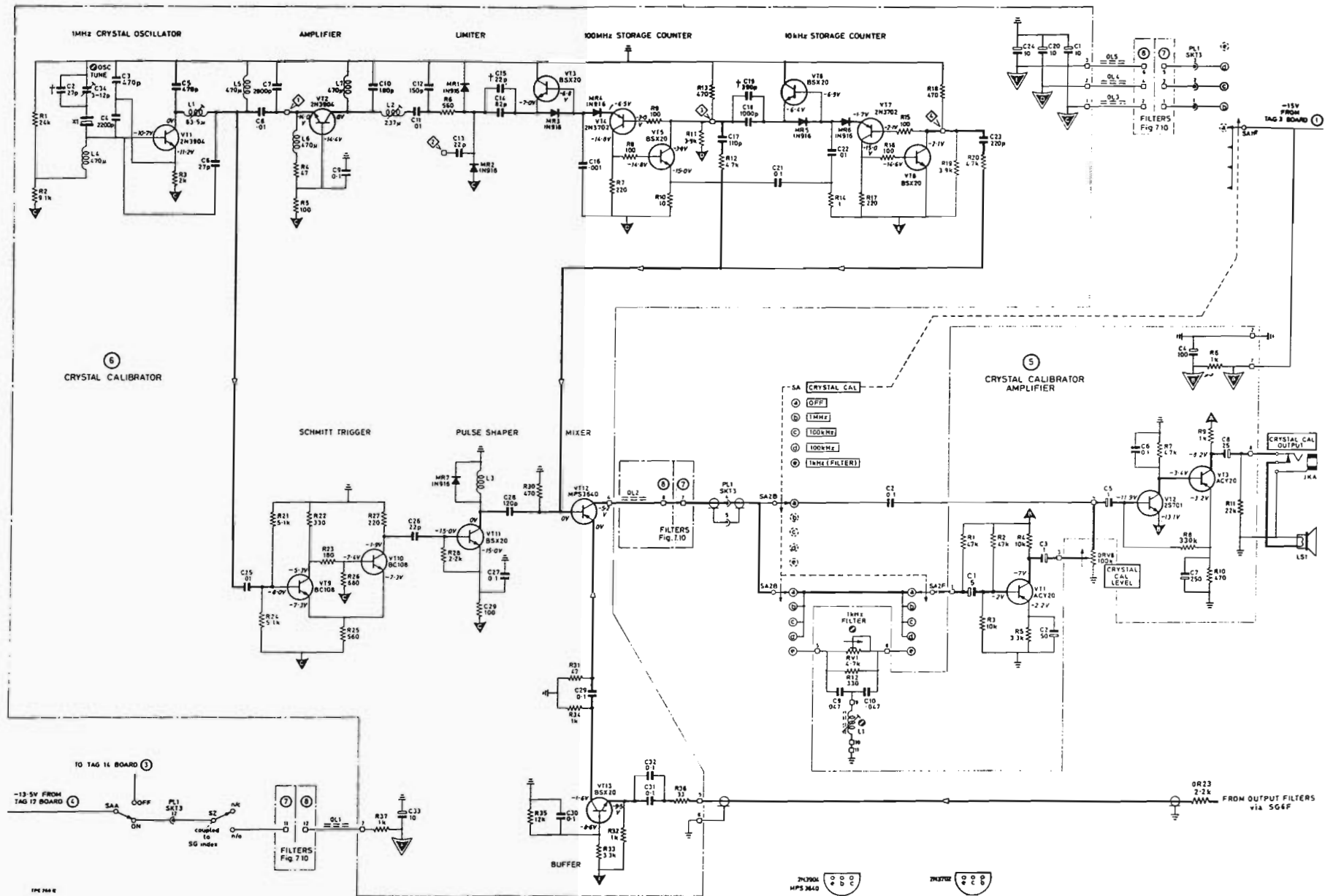
Fig. 7.8 Crystal calibrator
