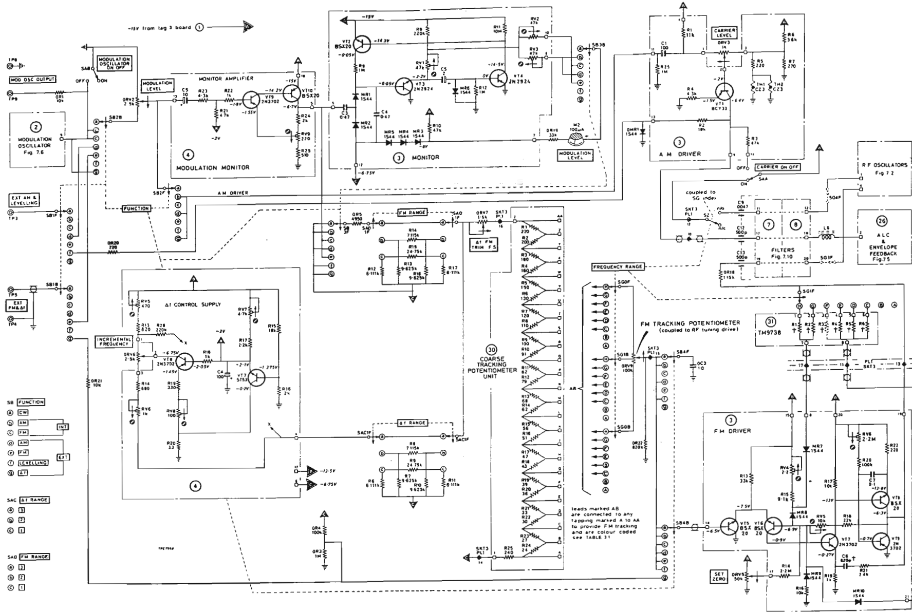
Fig. 7.7 A.M./F.M. drive and monitor
